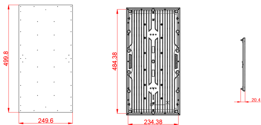
Graphite Module Dimensions (Unit: mm)
