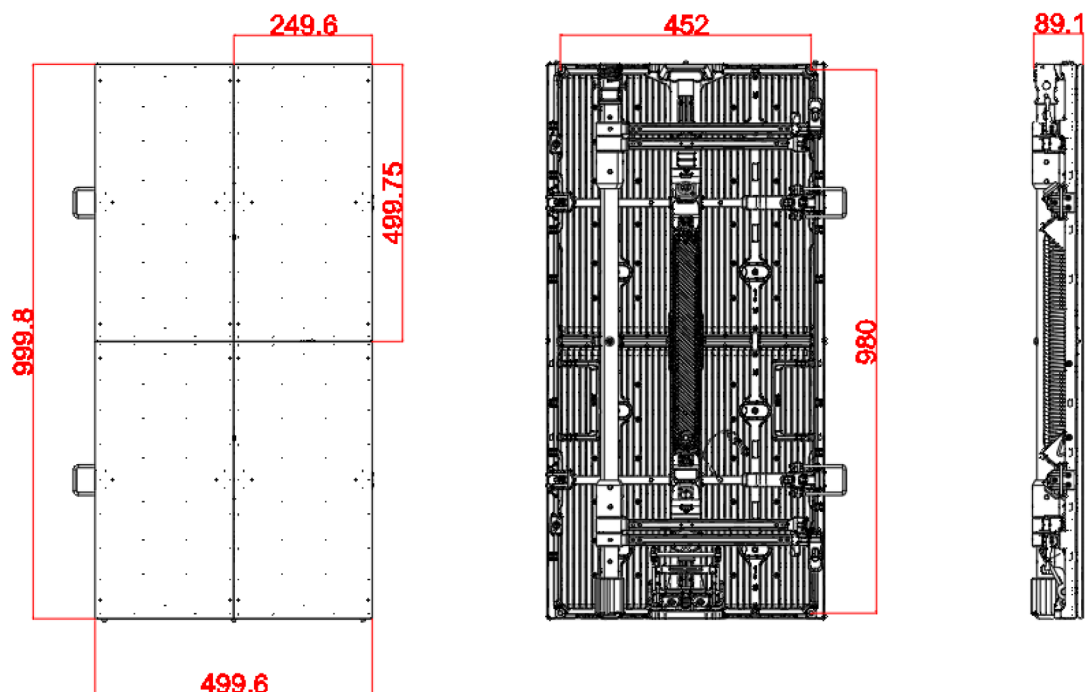
Graphite Panel Dimensions (Unit: mm)
